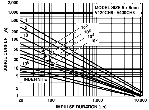
FIGURE 6. SURGE CURRENT RATING CURVES FOR V82CH8 - V430CH8
