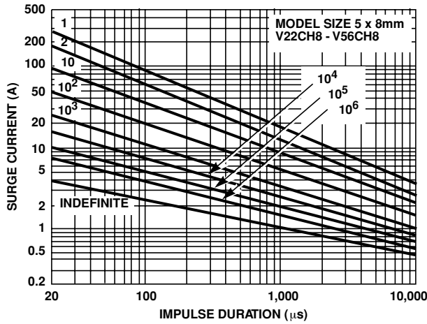
FIGURE 5. SURGE CURRENT RATING CURVES FOR V18CH8 - V68CH8
