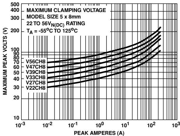
FIGURE 3. CLAMPING VOLTAGE FOR V18CH8 - V68CH8
