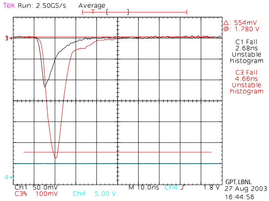
HFA1135 amplifier, 20 \Omega series output resistor, G-5.33, test pulse=300 Vdd=6.6V, Vss=-3.3V
