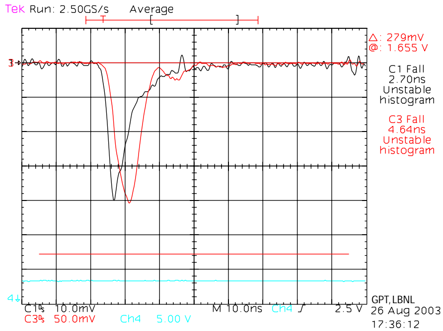
HFA1135 amplifier, 15 \Omega series output resistor, G-5.33, test pulse=300
