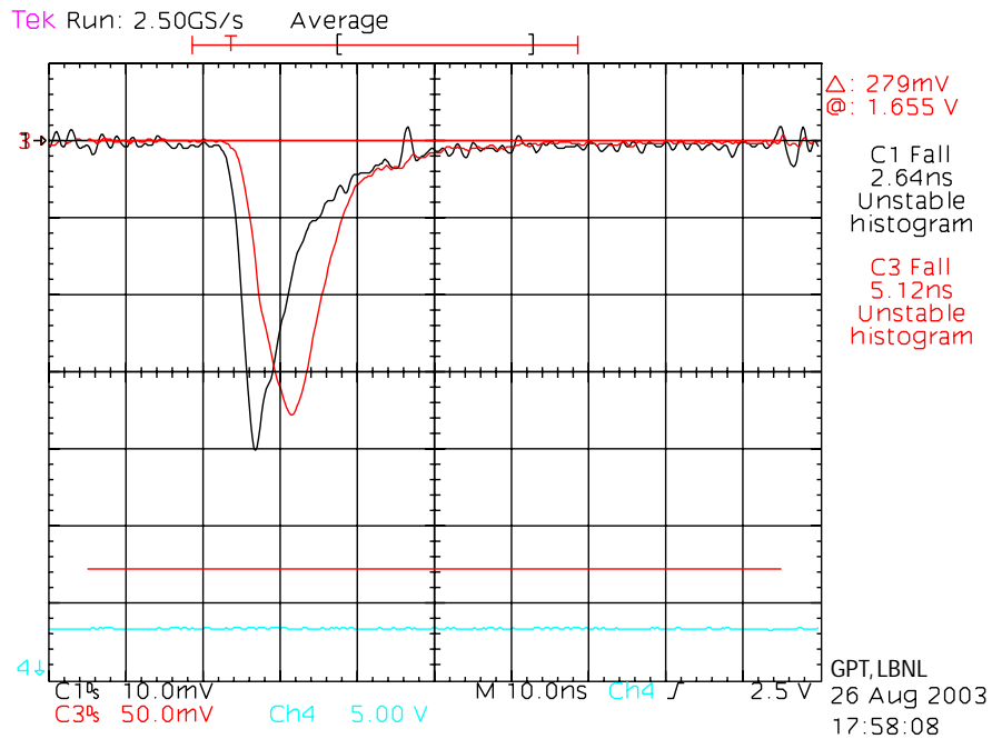
HFA1135 amplifier, 25 \Omega series output resistor, G-5.33, test pulse=300
