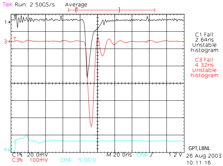
OPA689 amplifier, 10 \Omega series output resistor, G-8.0, test pulse=500
