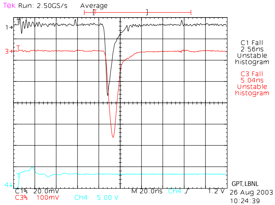
OPA689 amplifier, 25 \Omega series output resistor, G-5.33, test pulse=500
