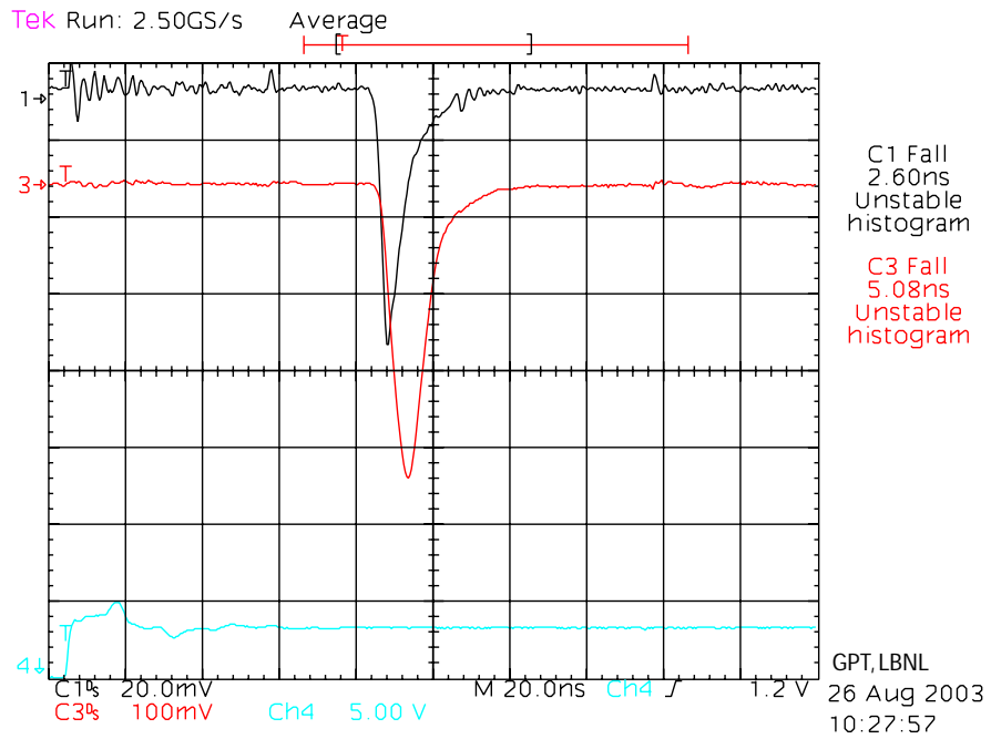
OPA689 amplifier, 30 \Omega series output resistor, G-8.0, test pulse=500
