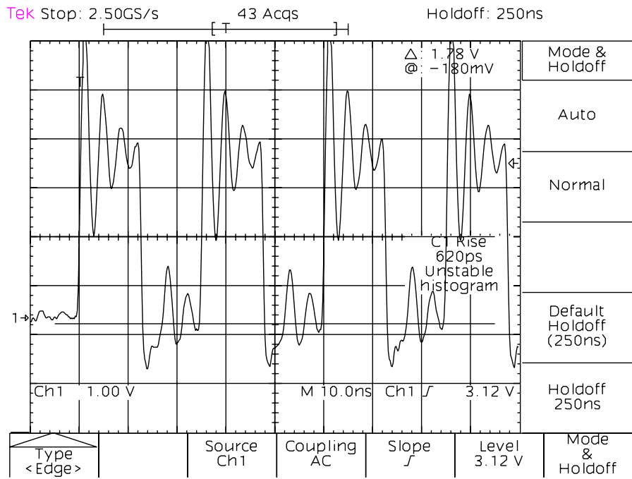
Counter Clock Buffer A Input, room temperature. gtp,tw,ag
