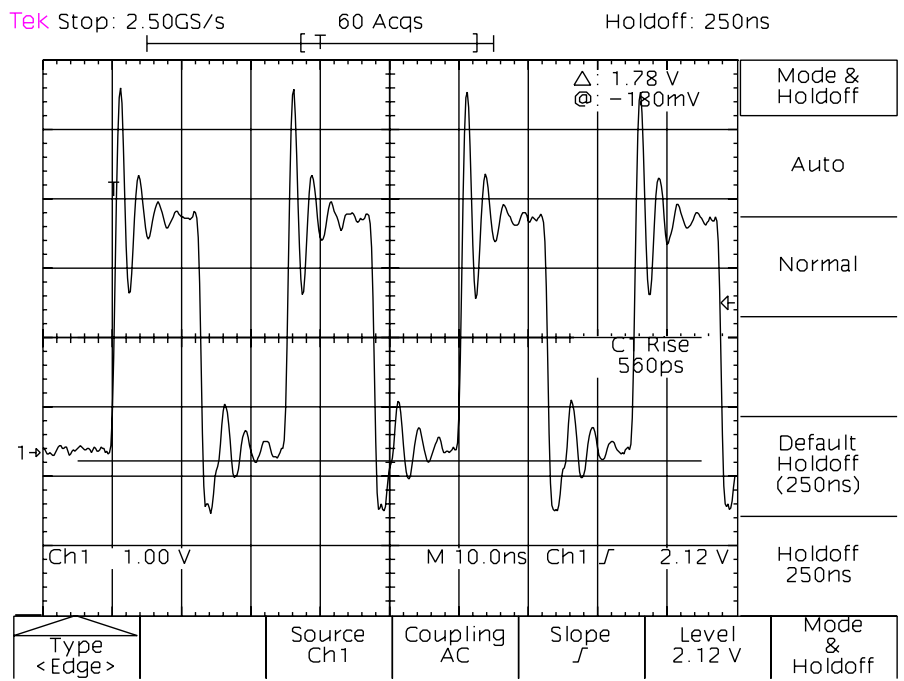
Counter Clock B Buffer Input, room temperature gtp, tw, ag
