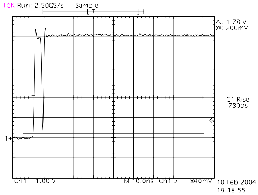
ATWD B Trigger Input Waveform, room temperature gtp, tw, ag
