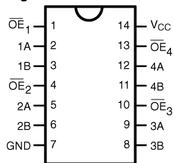
Pin Assignment for SOIC and TSSOP
