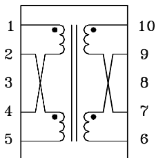
Circuit 1
