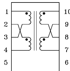
Circuit 2
