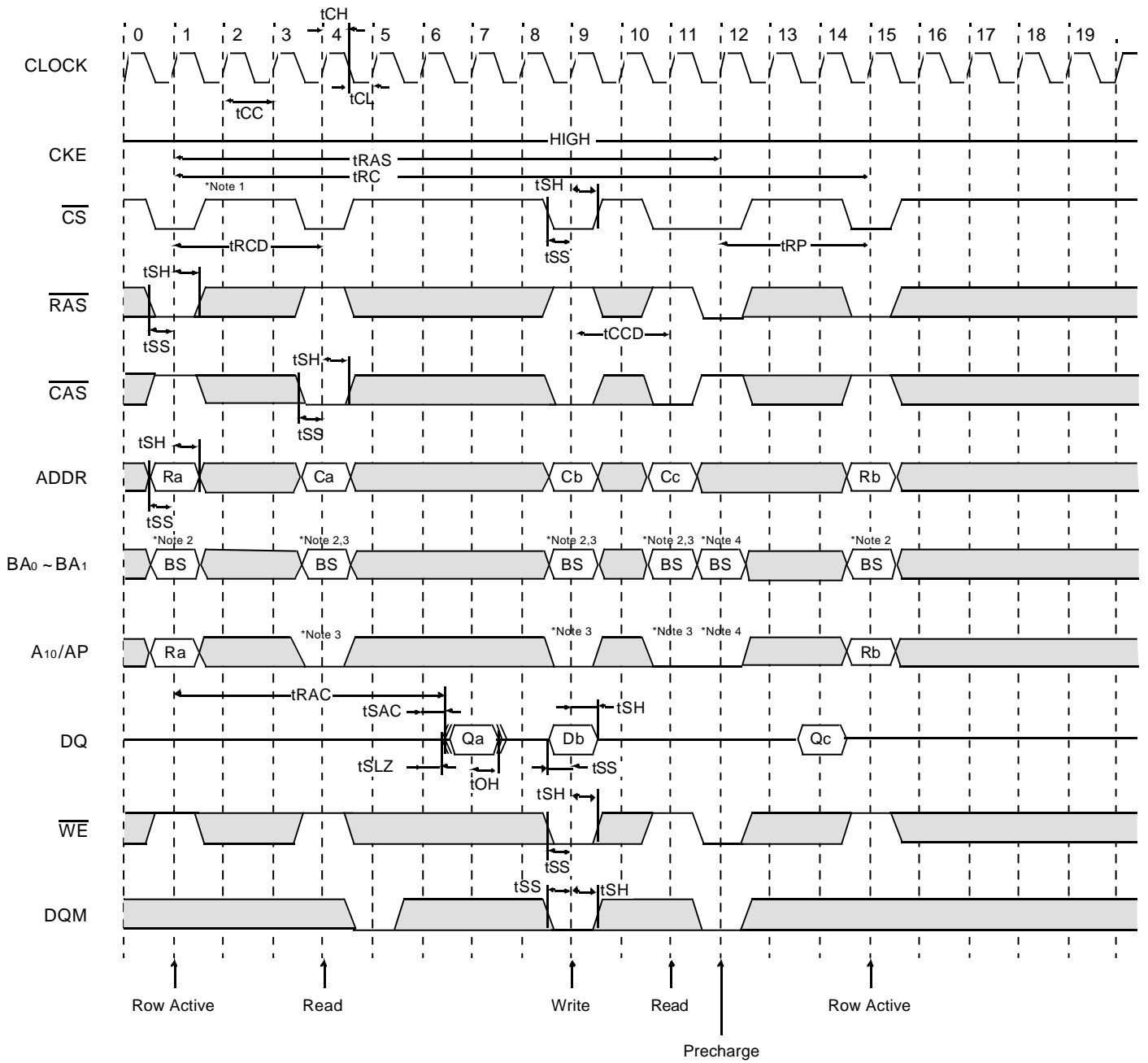
Single Bit Read-Write-Read Cycle(Same Page) @CAS Latency=3, Burst Length=1
