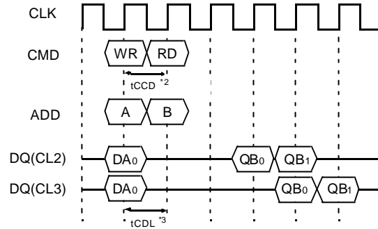
3) Write interrupted by Read (BL=2)
