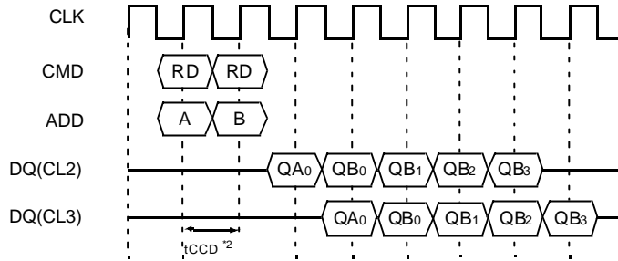
1) Read interrupted by Read (BL=4) *1
