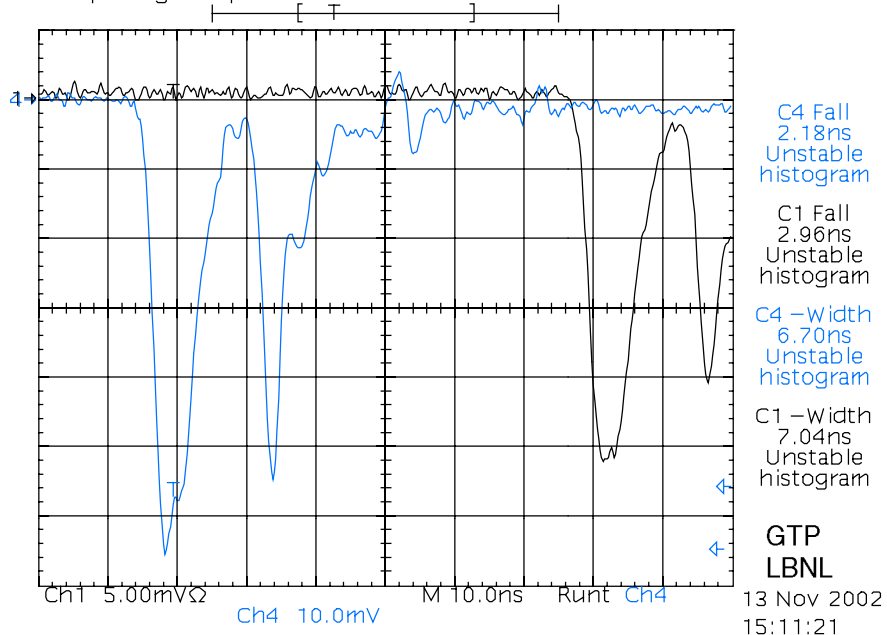
PMT Pulse into RG-62/U Coax Cable (Ch 1) and out (Ch 2). Pulse source: Burle 8575 Photomultiplier tube.
