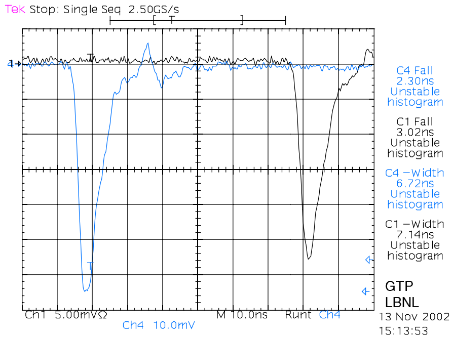
PMT Pulse into RG-62/U Coax Cable (Ch 1) and out (Ch 2). Pulse source: Burle 8575 Photomultiplier tube.
