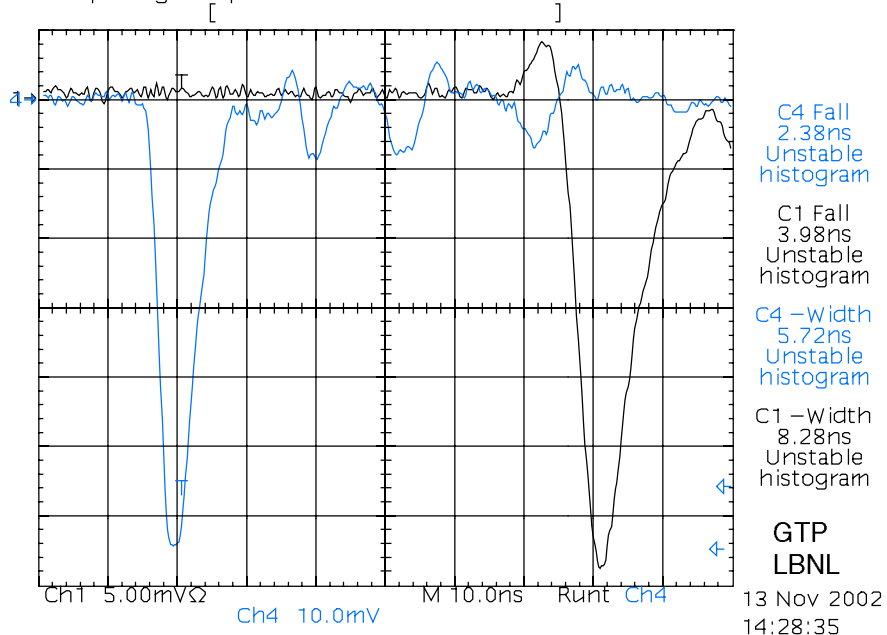
PMT Pulse into Lumped Delay (Ch 1) and out (Ch 2). Pulse source: Burle 8575 Photomultiplier tube.
