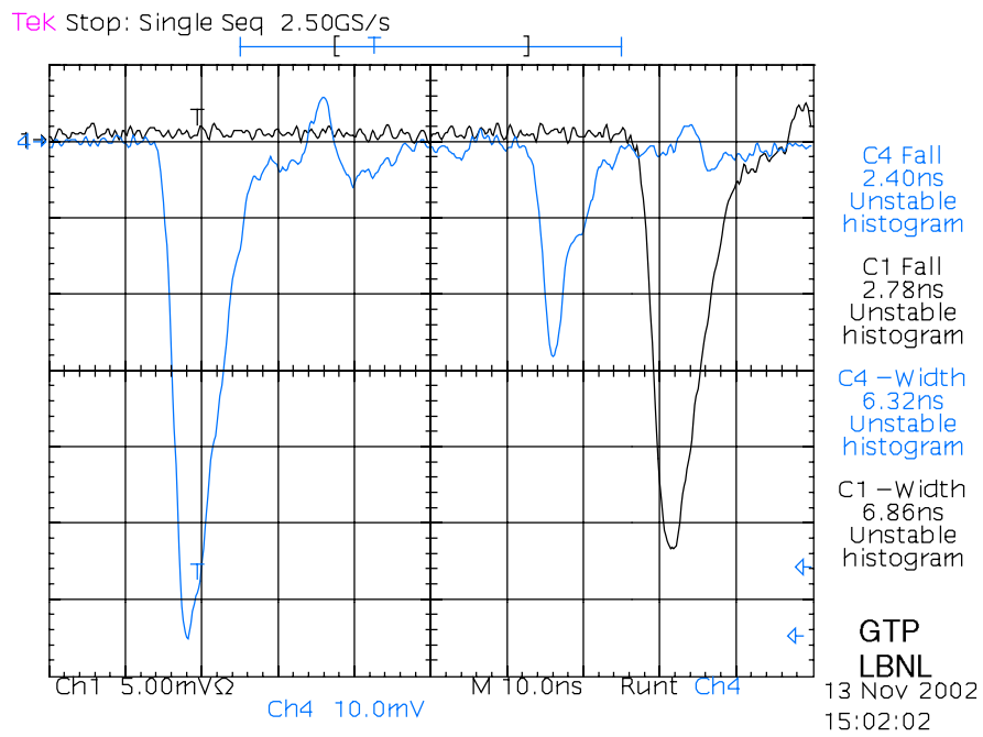
PMT Pulse into Lumped Delay (Ch 1) and out (Ch 2). Pulse source: Burle 8575 Photomultiplier tube.
