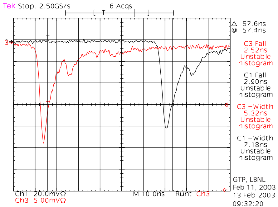
Waveform from Burl moeel 8575 Photomultiplier tube. The cursor shows a delay of about 57 ns
