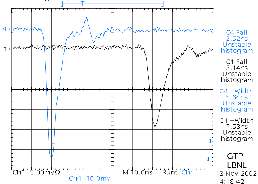
PMT Pulse into PCB Strip-Line Delay (Ch 1) and out (Ch 2). Pulse source: Burle 8575 Photomultiplier tube.
