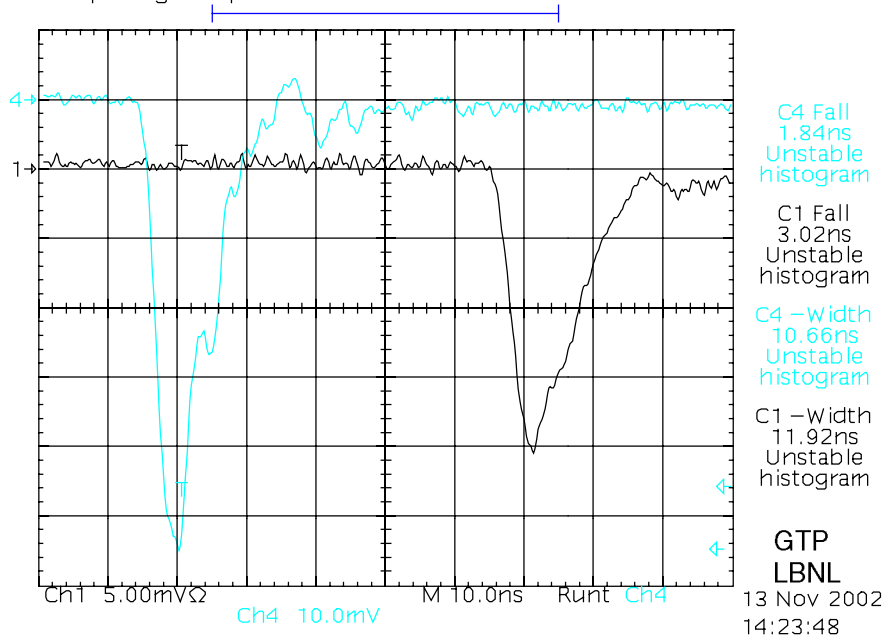
PMT Pulse into PCB Strip-Line Delay (Ch 1) and out (Ch 2). Pulse source: Burle 8575 Photomultiplier tube.
