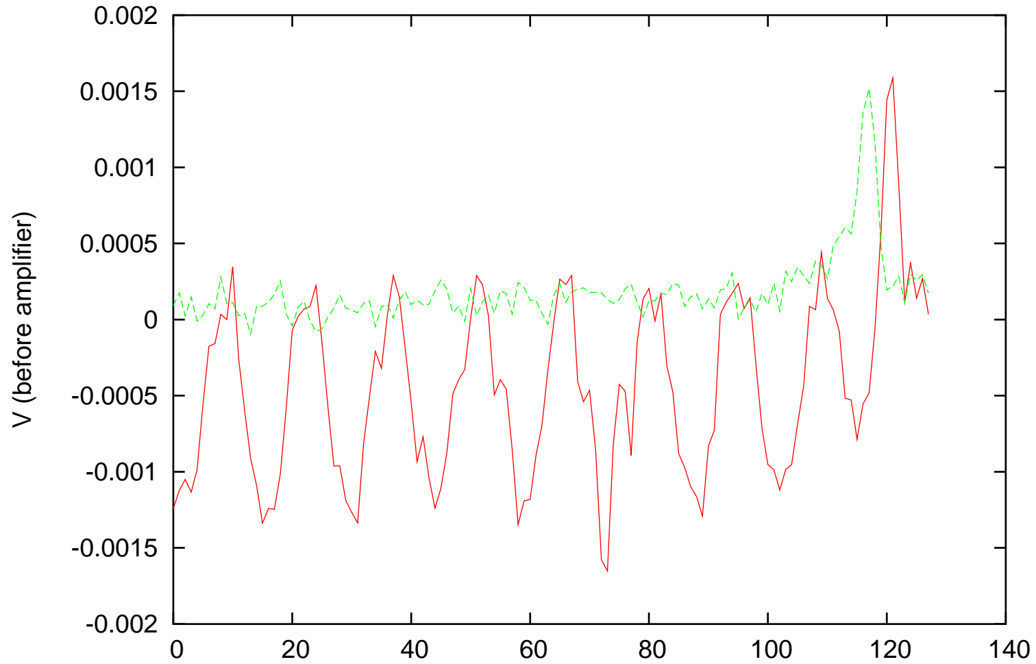
ATWD Noise With/Without Oscillator into Ch3
