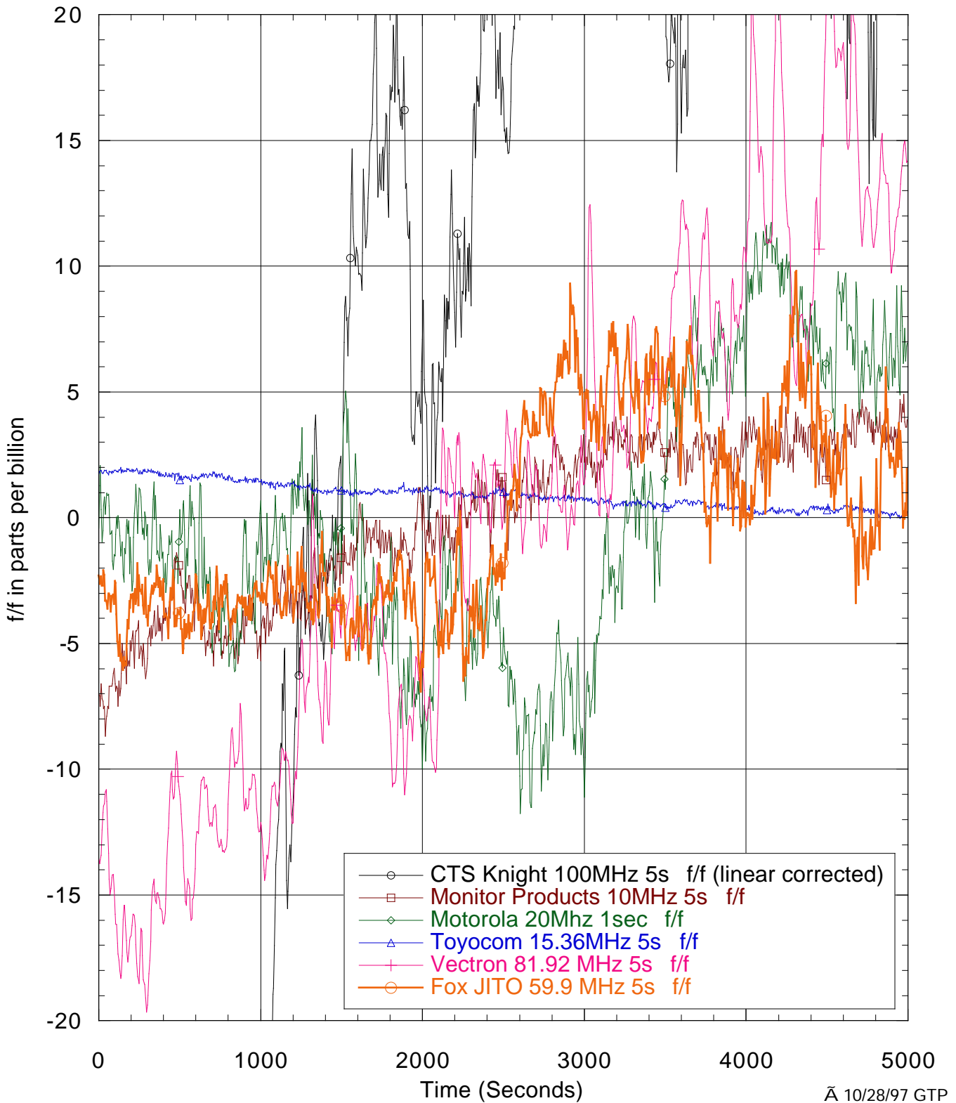
Short term stability tests for samples of low cost oscillators from various manufacturers. This survey was not exhaustive. No product exceeded $100 in cost per unit. All products except Fox were off-the-shelf.
